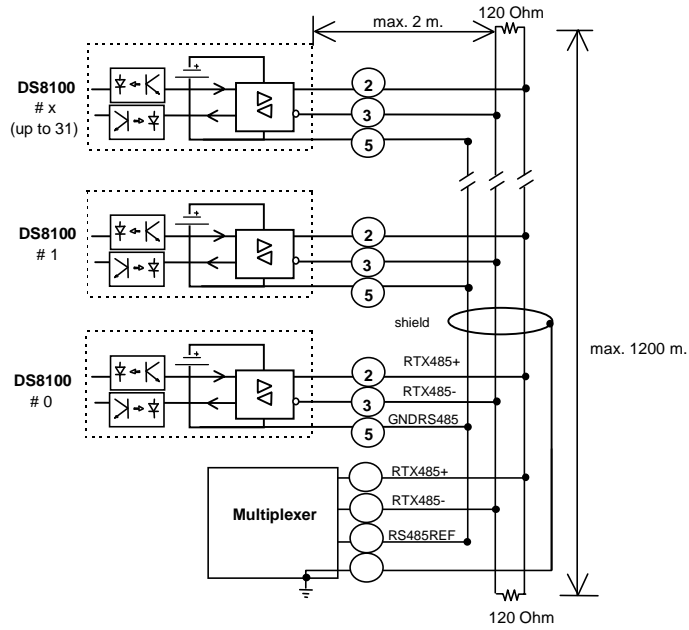
Figure 2.13 - DS8100 Multidrop connection to a Multiplexer
