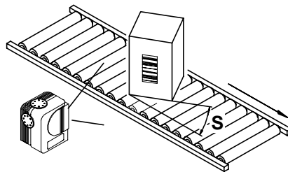
Figure 3.7 - "Skew" angle
