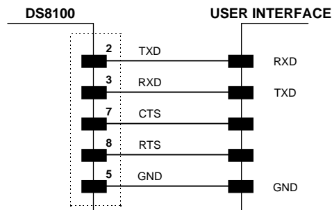
Figure 2.10 - RS232 connections
