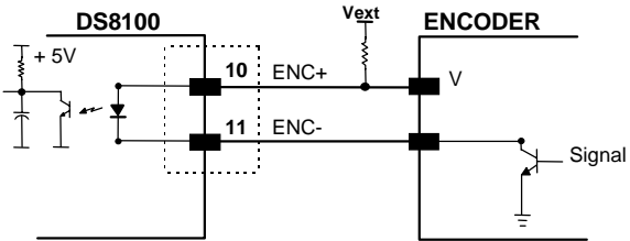
Figure 2.21 - Encoder NPN input command using external power
