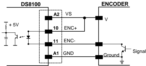
Figure 2.20 - Encoder NPN input command using DS8100 power
