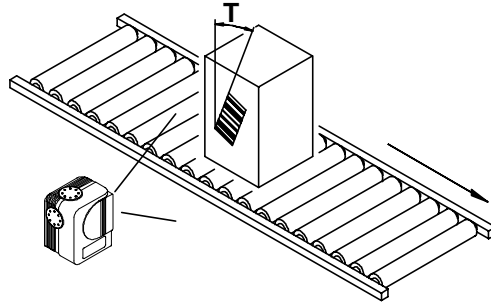
Figure 3.8 - "Tilt" angle
