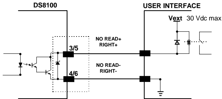
Figure 2.24 - Output interface
