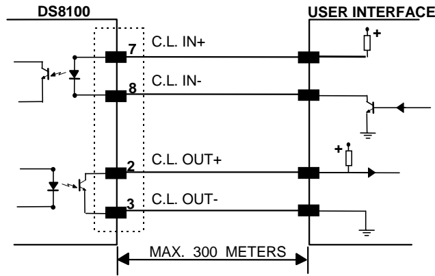
Figure 2.15 - 20 mA C.L. passive connections
