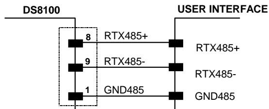
Figure 2.17 - RS485 Auxiliary interface connections
