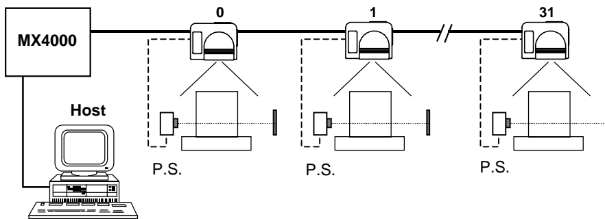
Figure 2.32 - Multiplexer layout
