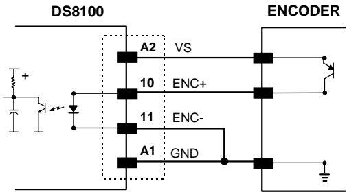
Figure 2.22 - Encoder PNP input command using DS8100 power
