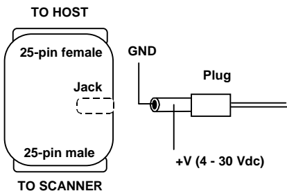
Power supplied using the jack connector
