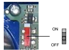
Figure 8 – ID-NET™ Termination Resistance Switch
