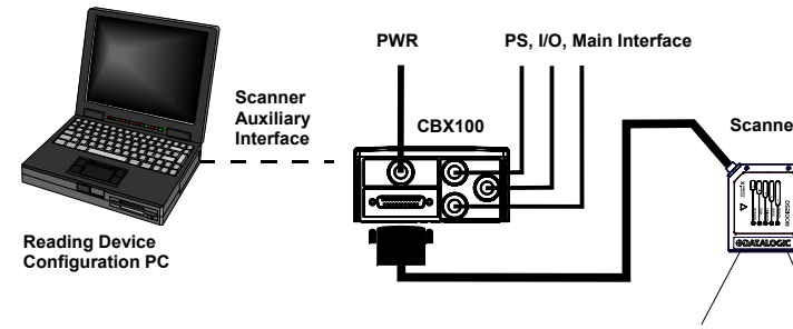
Figure 2 - System Layout
