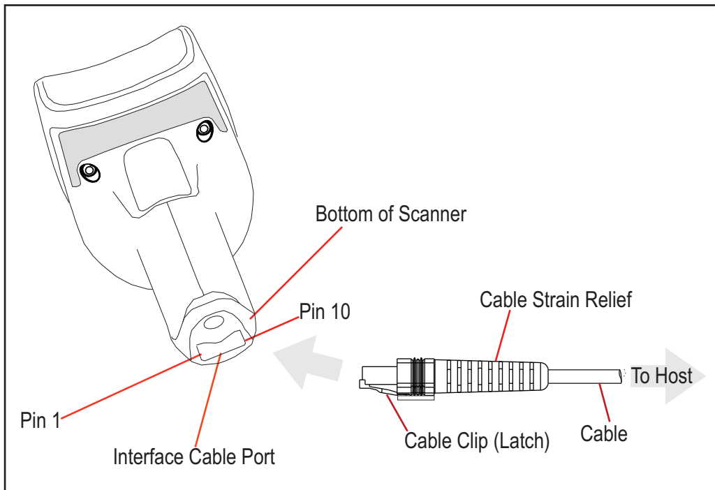
Figure 10. Standard Cable Pinouts: Handheld
