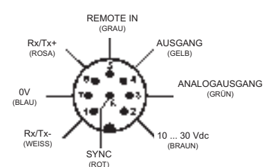
8-POLIGER M12-STECKER
